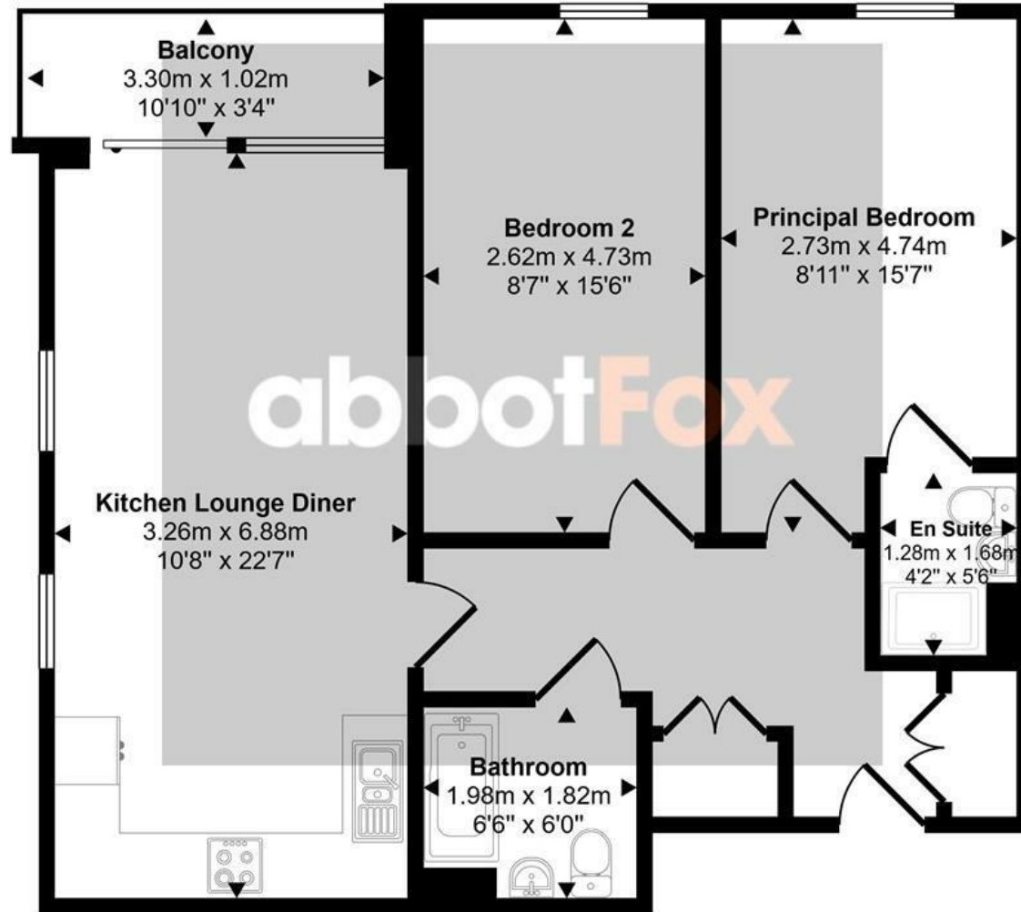
Floorplan
